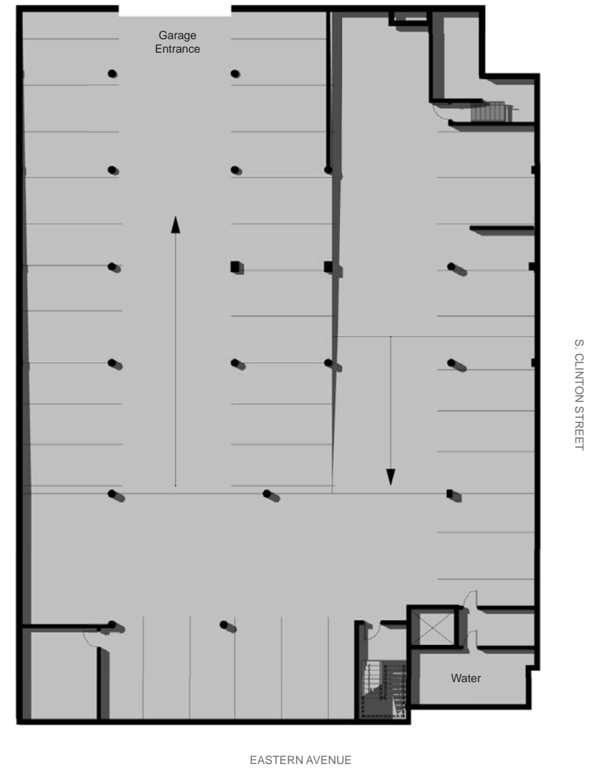
Basement Level UDARP Schematic Presentation Dec 17, 2015
