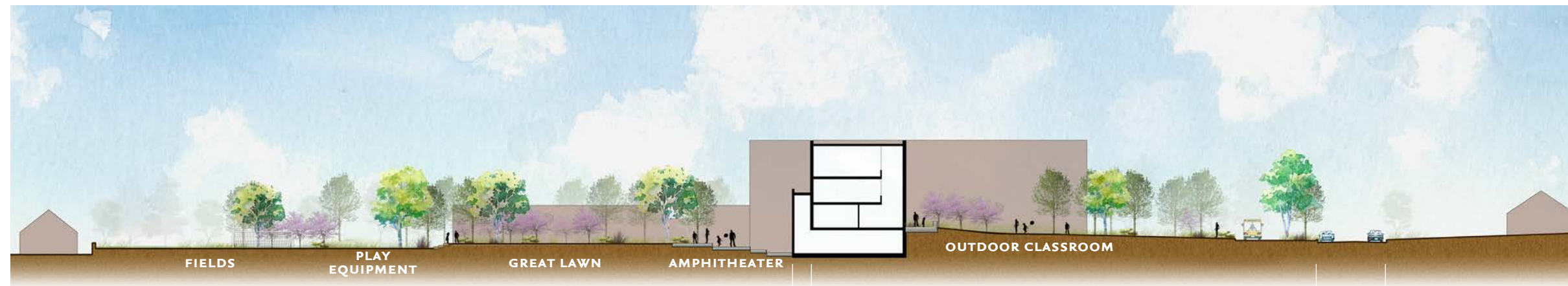
SECTION C FIELDS PLAY EQUIPMENT GREAT LAWN AMPHITHEATER BUILDING ADDITION OUTDOOR CLASSROOM W ROGERS AVENUE
