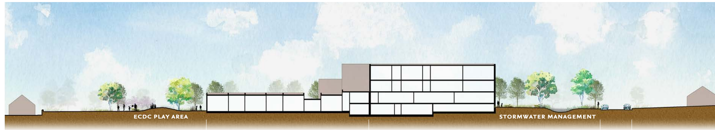
SECTION B ECDC PLAY AREA ECDC ADDITION STORMWATER MANAGEMENT W ROGERS AVENUE
