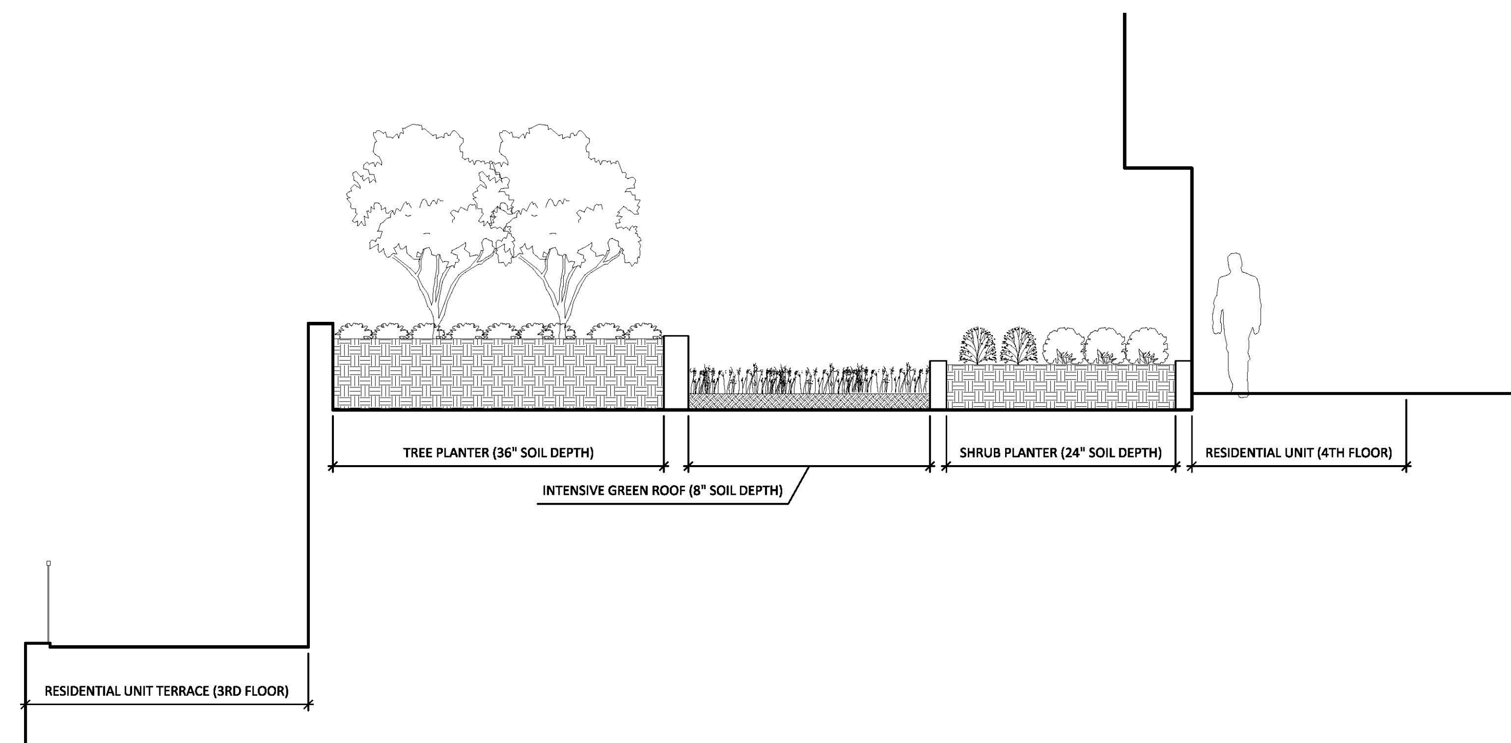
1 SECTION A-A' 1/4" = 1'-0"
