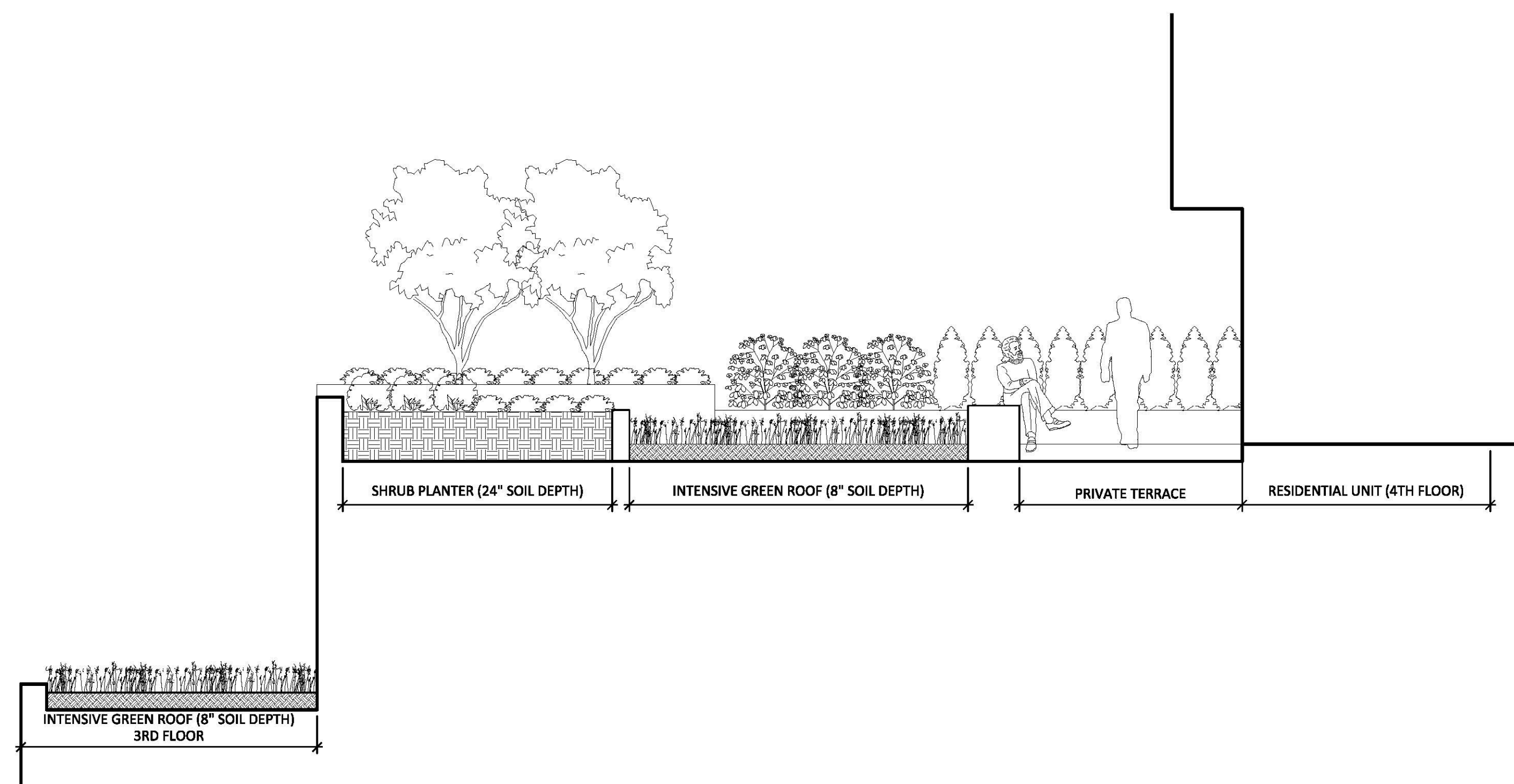
2 SECTION B-B' 1/4" = 1'-0"
