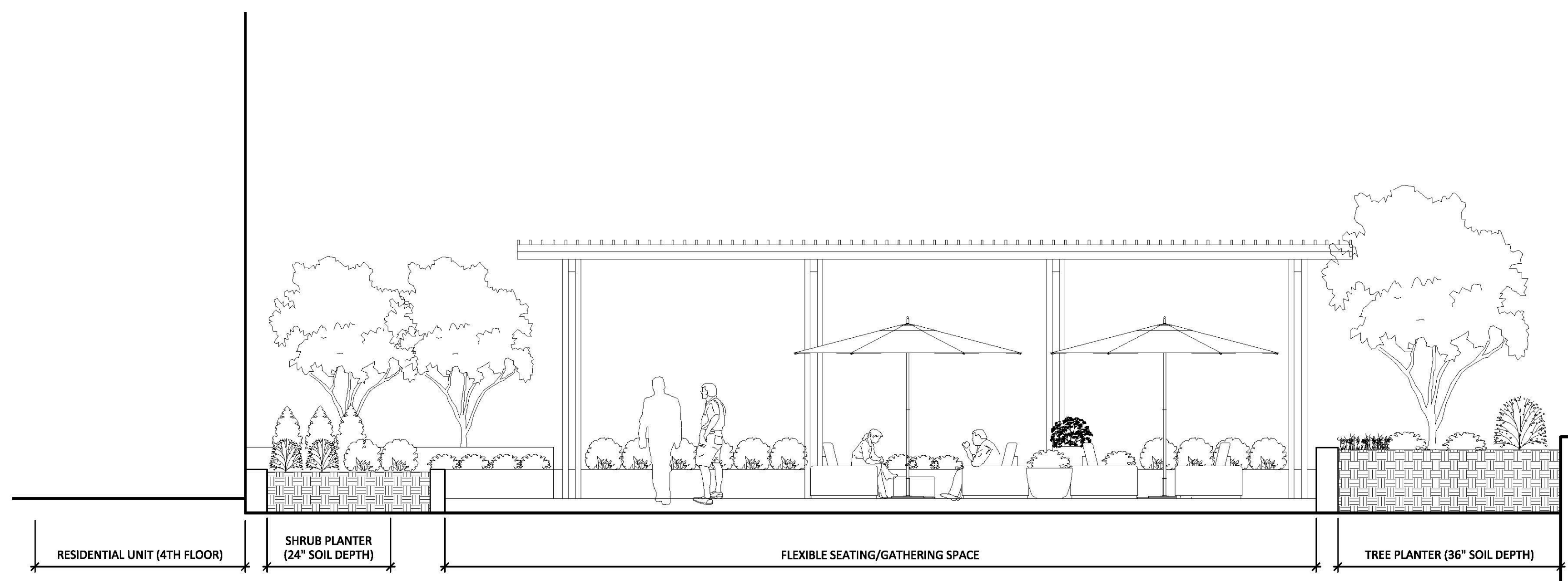
5 SECTION E-E' 1/4" = 1'-0"
