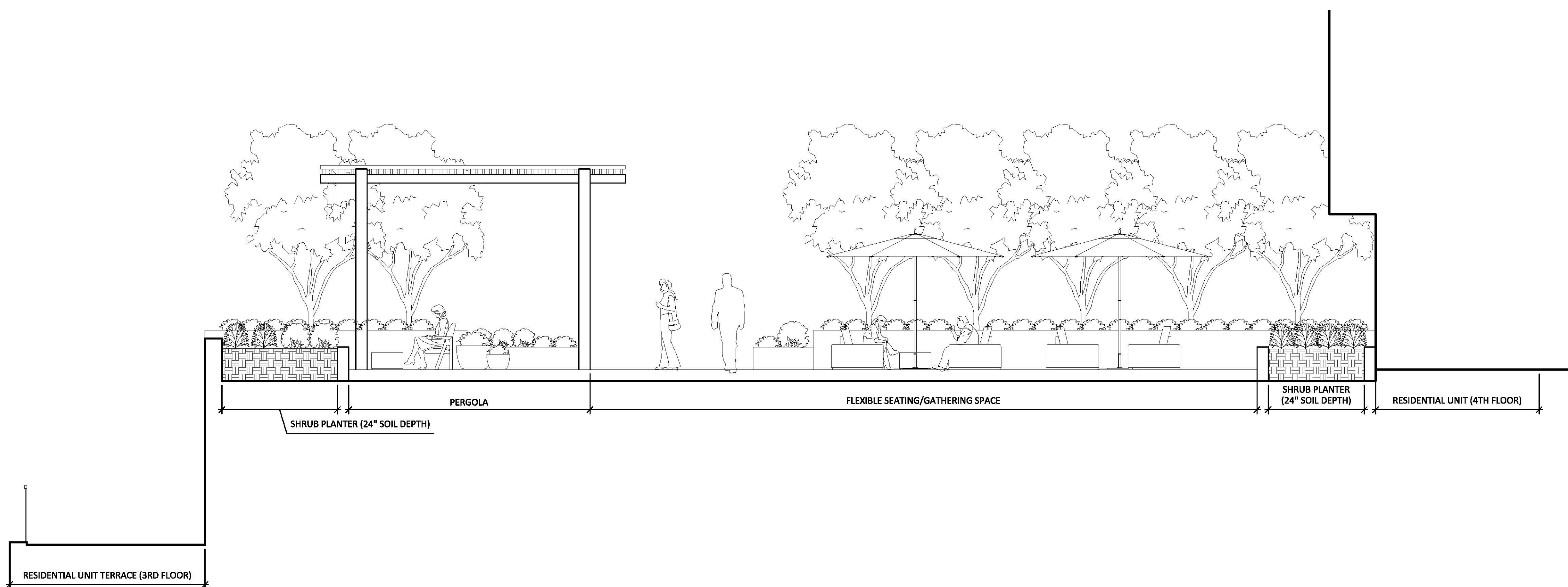
3 SECTION C-C' 1/4" = 1'-0"
